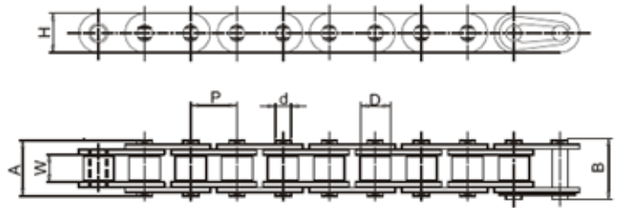
STRAIGHT SIDE PLATE CHAINS - EUROPEAN SERIES
