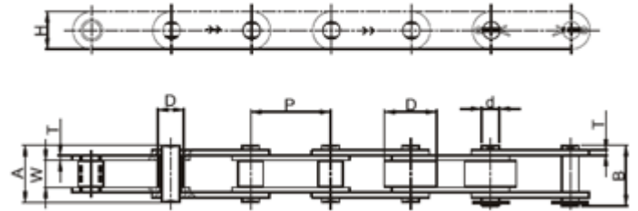
STAINLESS STEEL CHAINS DOUBLE PITCH AMERICAN SERIES - CONVEYOR
