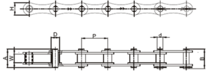
STAINLESS STEEL CHAINS DOUBLE PITCH - AMERICAN SERIES
