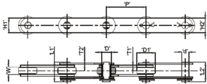
METRIC SERIES (ISO) - SOLID PIN CHAINS
